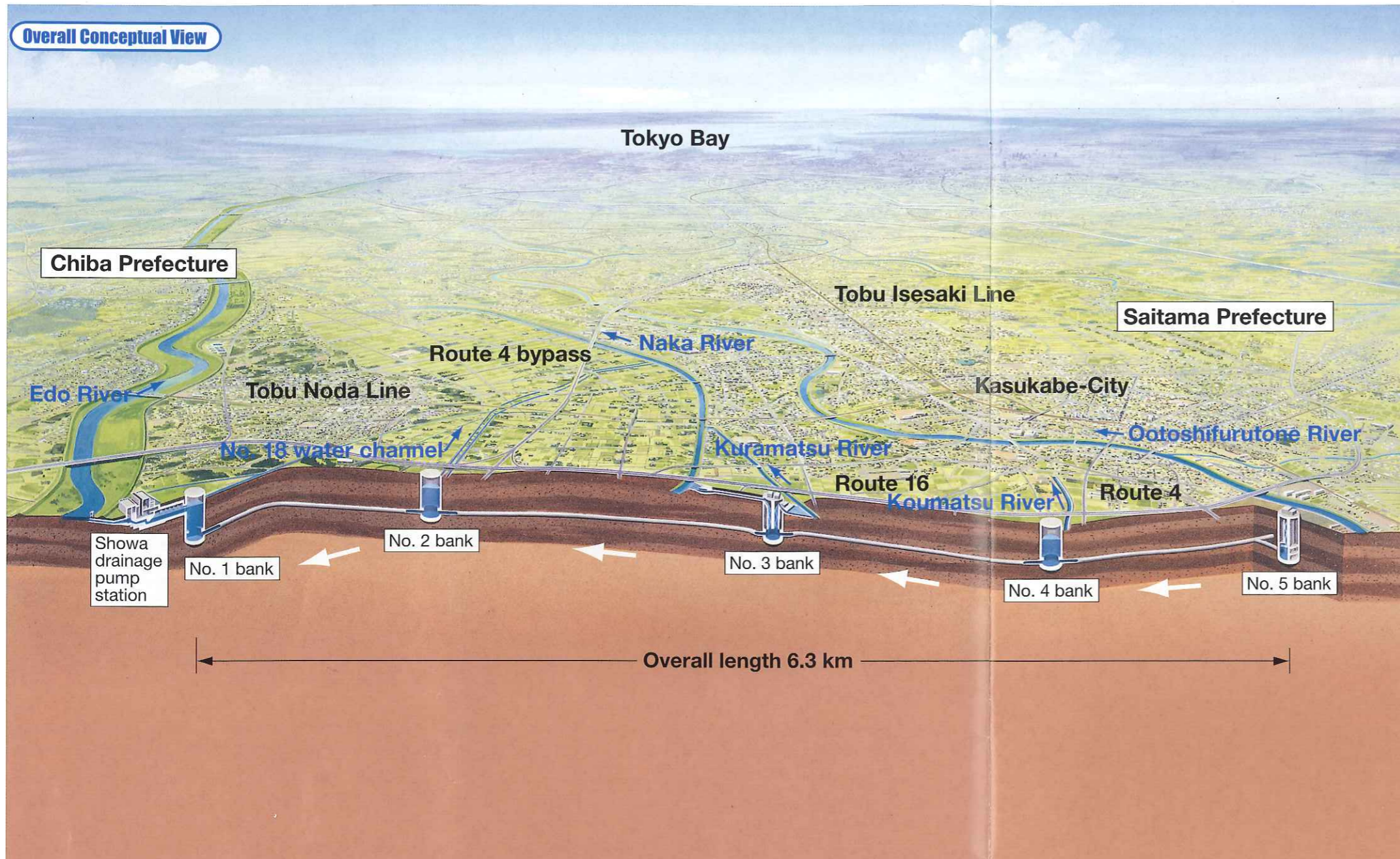
Showa Drainage Pump Station
