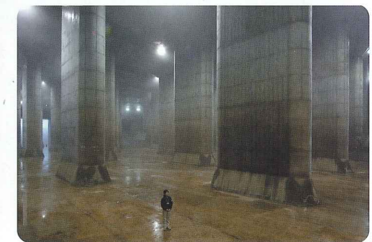
Pressure-adjusting water tank
